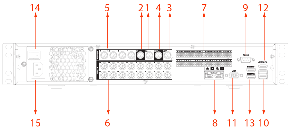
Figure 3-20 Rear panel (3)
