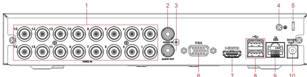
Figure 3-21 Rear panel
